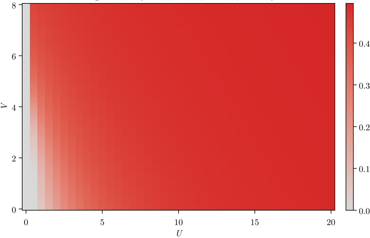
Magnetization ( t = 1.0 , L = 128 , \delta = 0.0 , \beta = 100.0 )
